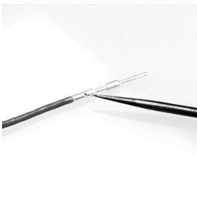
1. Insert stripped wire into contact pocket until it is visible through inspection hole.
