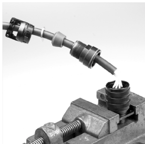
13. Plug with all contacts inserted, check that all contacts are fully seated.
