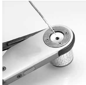
2. Fully seat contact in crimping tool.
