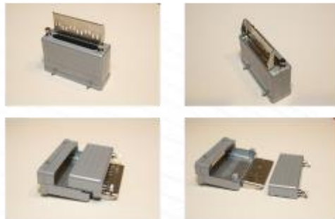
Amphenol Tel-Ad custom hood, easy for maint Custom made cord grip.
